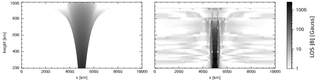
Fig. 1. Result of the accuracy test of the proposed hybrid bisector-COG method. Left: input model. Right: recovered flux density. The height scale for the recovered flux density was derived using calculations of \tau_\lambda = 1 . The gray scale encodes the magnetic flux density and is the same for both panels.
